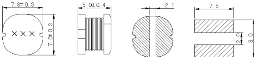
Land Pattern
